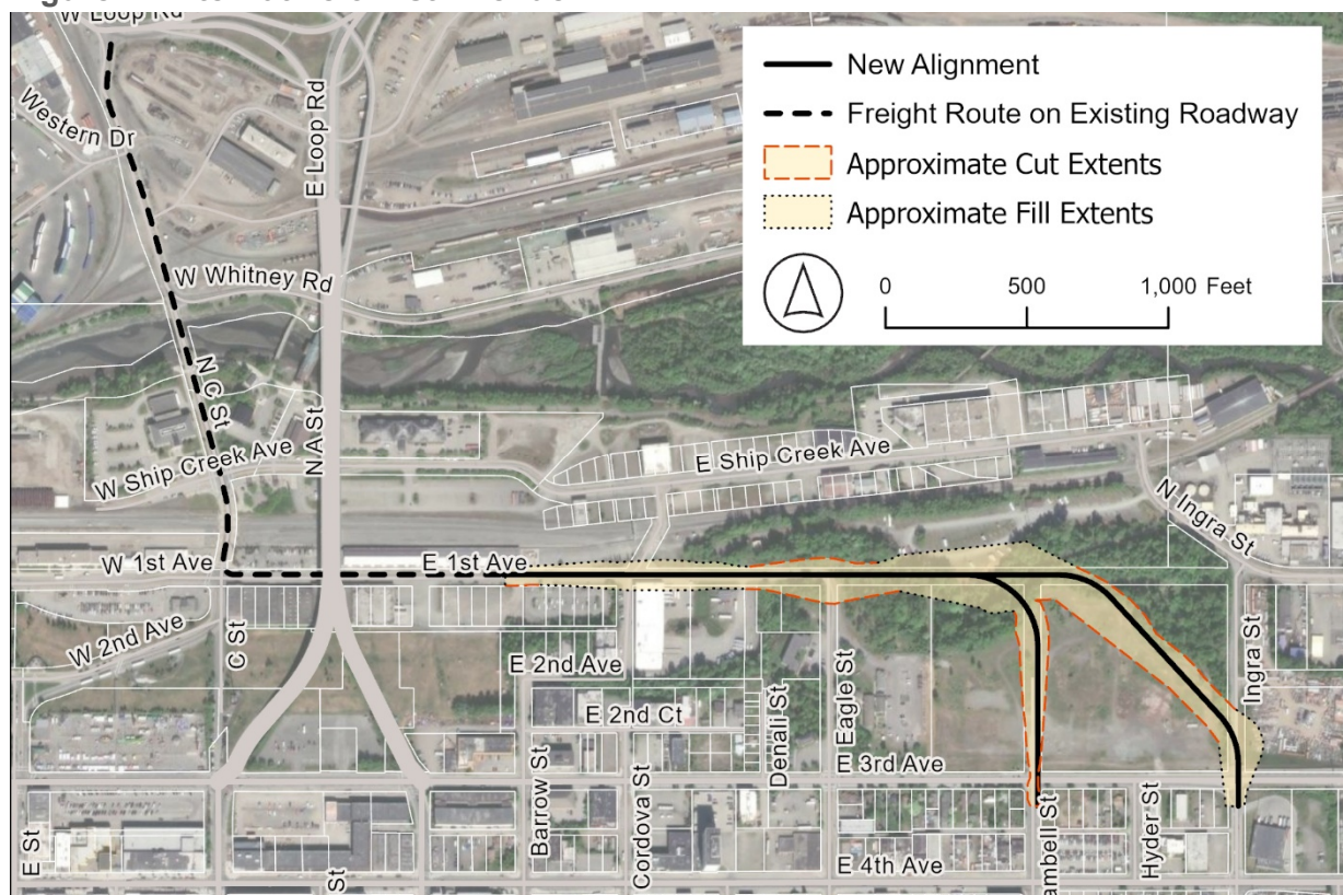
Figure 7: Alternative 3: 1st Avenue
