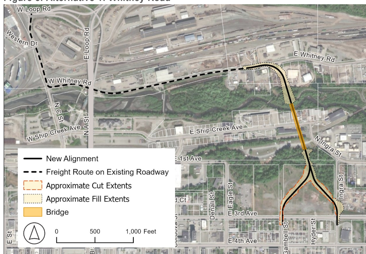
Figure 5: Alternative 1: Whitney Road
