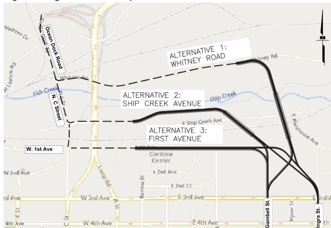
Figure 4: Ingra-Gambell Couplet Extension Alternatives
