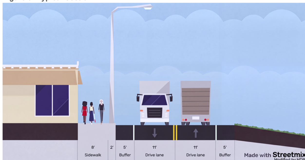
Figure 9: Typical Section
